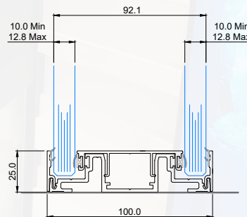
DOUBLE GLAZED FLOOR TRACK
