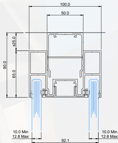
DOUBLE GLAZED HEAD TRACK ± 25MM DEFLECTION
