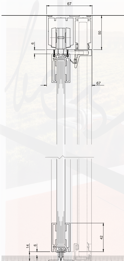
SECTION THROUGH SINGLE GLAZED KINETIC ALIGN SLIDING DOOR NO DEFLECTION
